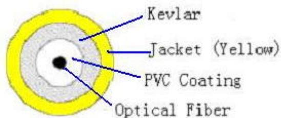
Figure 2 Cable section
